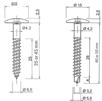
UNI Screw with standard tip
