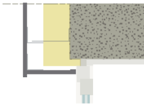
Figure 14: Jamb Detail
